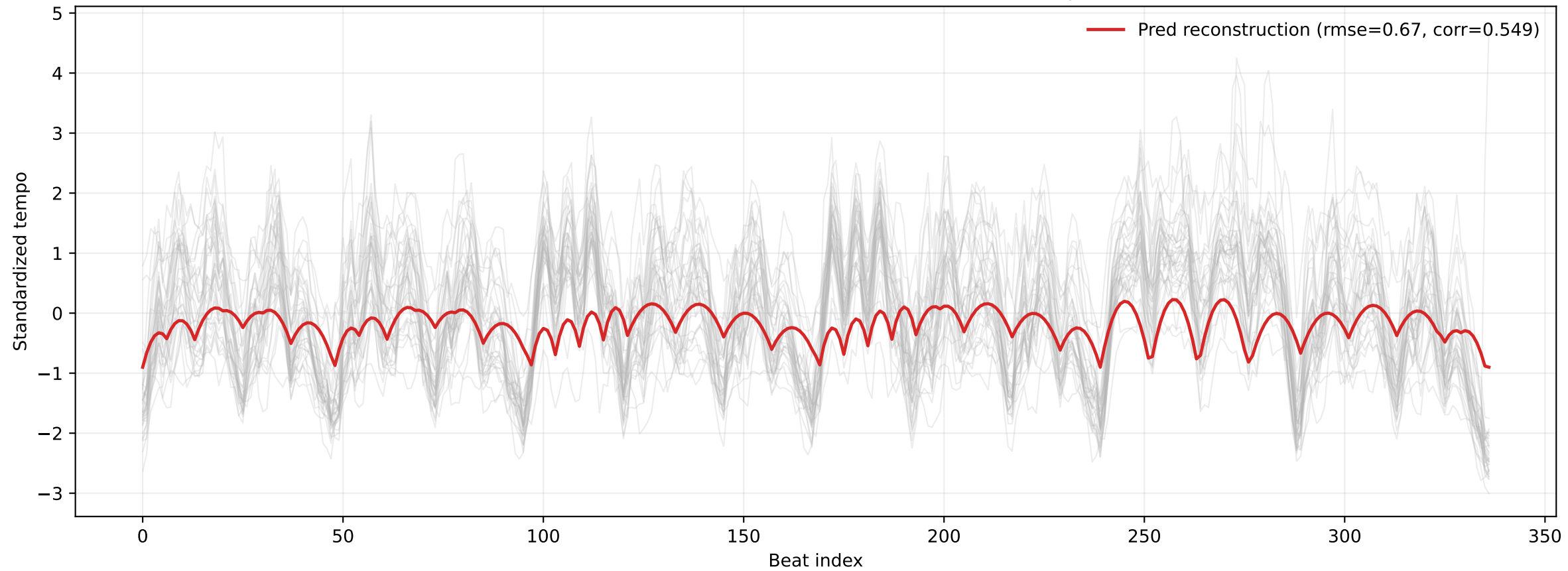
M06-1: Pred reconstruction vs ALL standardized true tempo curves
